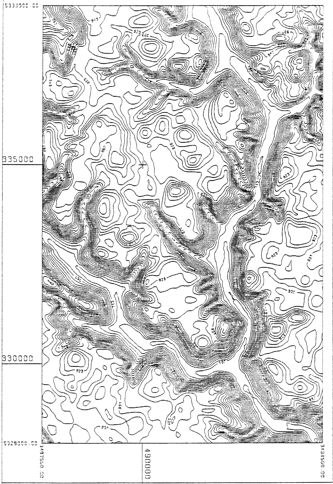
APPENDIX 2: Contour representation of the DEM
