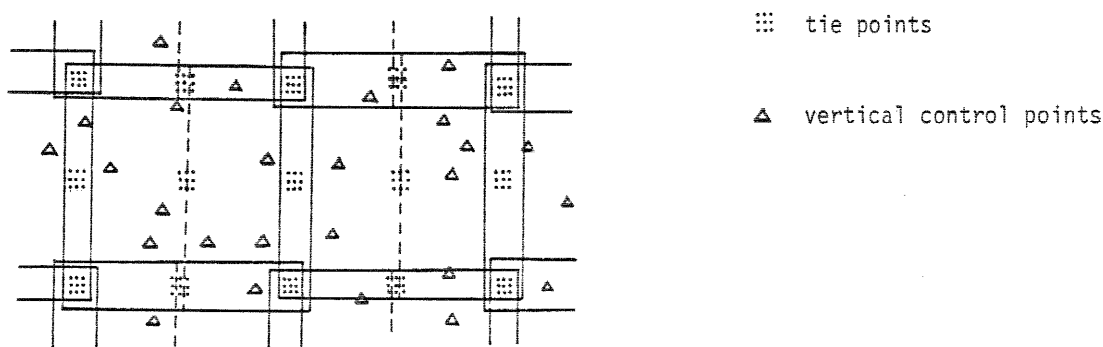
Fig. 2: Point distribution for the vertical block adjustment
