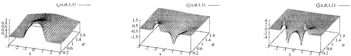
Figure 2: Scale-space behaviour of the bar-shaped line f_b when convolved with the derivatives of Gaussian kernels for x \in [-3, 3] and \sigma \in [0.2, 2]
