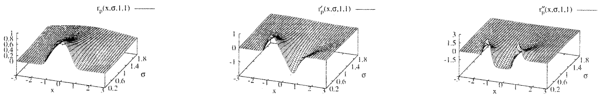
Figure 1: Scale-space behaviour of the ideal line f_p when convolved with the derivatives of Gaussian kernels for x \in [-3, 3] and \sigma \in [0.2, 2]
