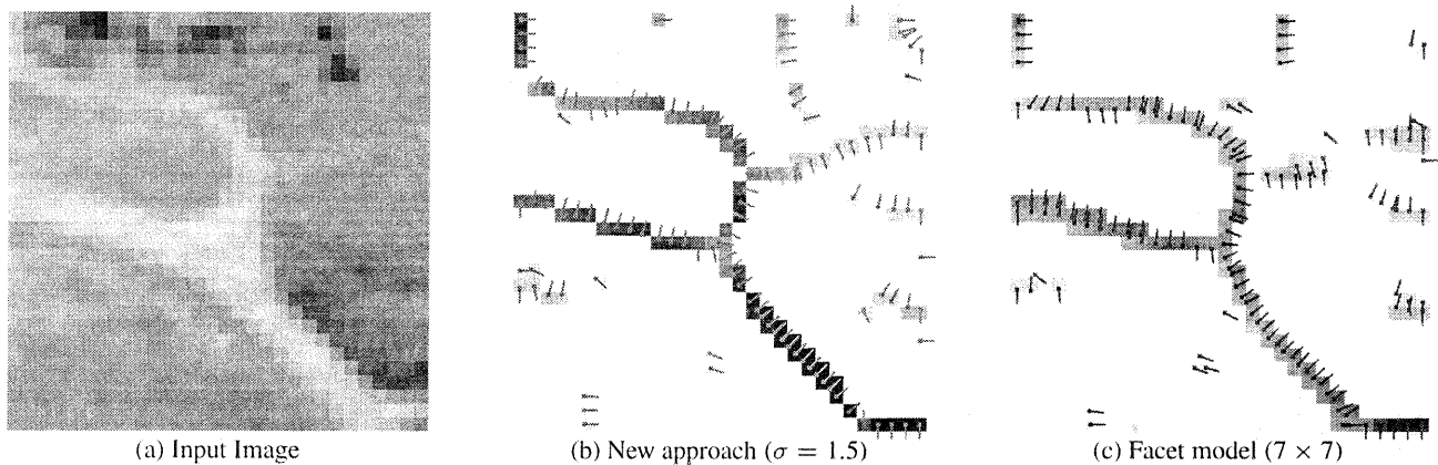
Figure 4: Line points detected in image (a) using the new approach (b) and using the facet model (c)
