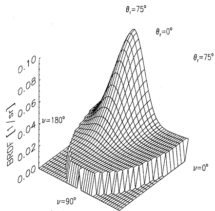
Figure 8: BRDF of the sample 'slate' at \theta_i = 25^\circ and \lambda = 850 nm
