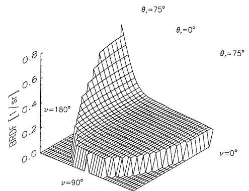
Figure 4: BRDF of the Spectralon panel at \theta_i = 75^\circ and \lambda = 850 \text{ nm}
