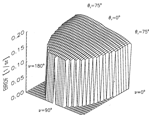
Figure 3: BRDF of the Spectralon panel at \theta_i = 25^\circ and \lambda = 850 \text{ nm}
