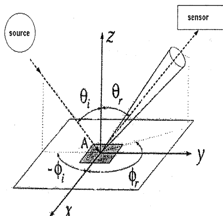
Figure 1: Definition of the angles A denotes the surface of the sample
