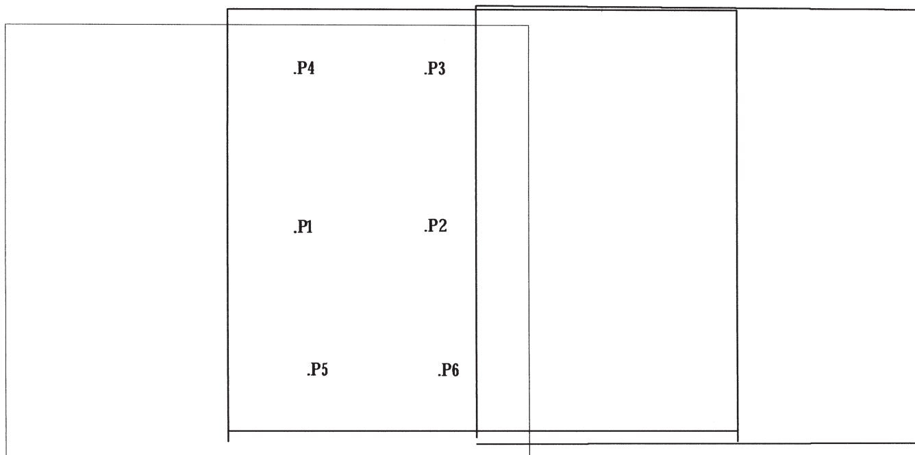
Figure 2: A Typical Photogrammetry R0 Point Selection Schema
