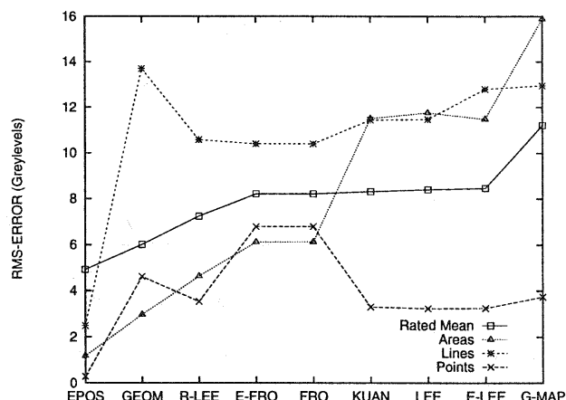
Figure 2: Distortions at geometric primitives (CONT = 100)
