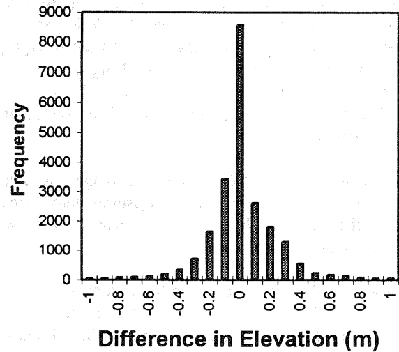
Figure 4. The frequency of points within the WisDOT DTM with a given difference in elevation between the WisDOT DTM and the Leica DEM.
