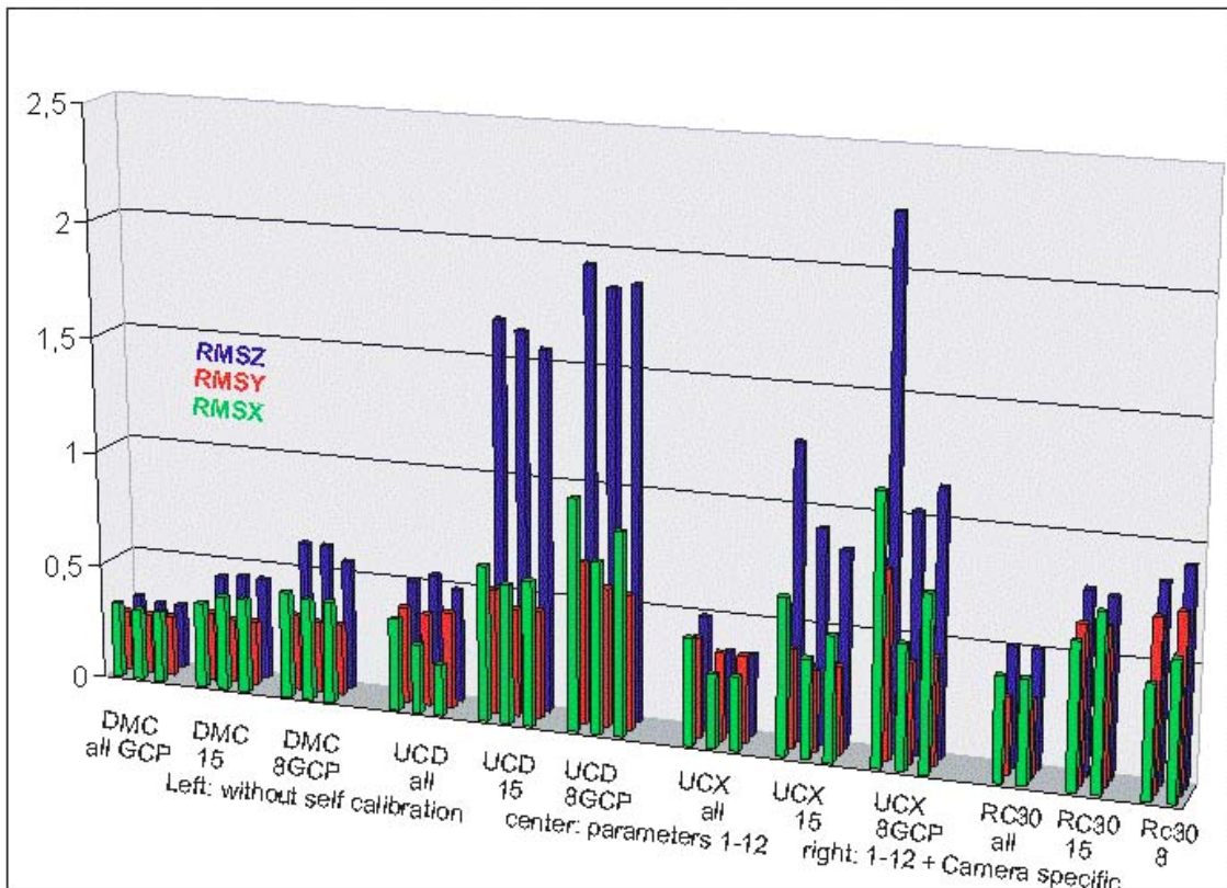
Fig. 9: comparison of achieved results in Franklin Mills [GSD]
