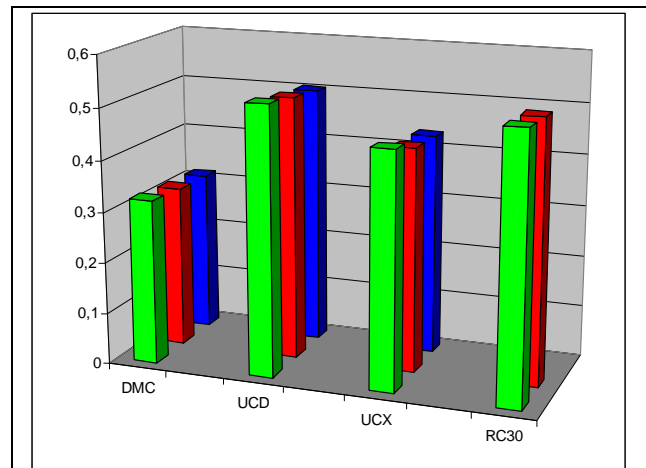
Fig. 8: standard deviations of unit weight sigma0 [pixels] First column (green): without self calibration Second column (red): self calibration with parameters 1 – 12 Third column (blue): self calibration with parameters 1 – 12 + camera specific parameters
