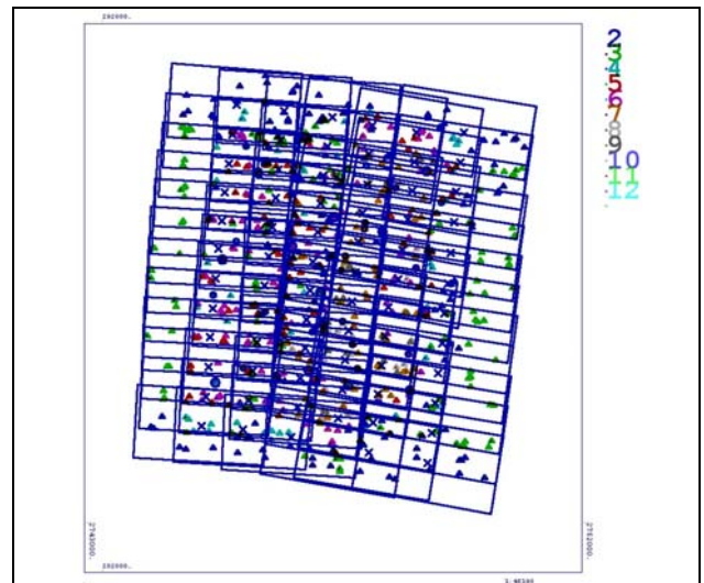
Fig. 3: DMC-block Franklin Mills with colour coded number of images / object points – colour scale see upper right
