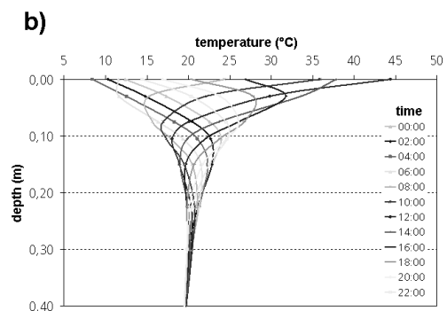
Figure 2. Two examples of modelled soil temperatures for one day. (a) shows the development of soil temperatures at 1cm, 5cm, 20cm and 80cm depth, (b) shows temperature profiles for various times. Damping and phase shift of the diurnal surface temperature wave are clearly visible.
