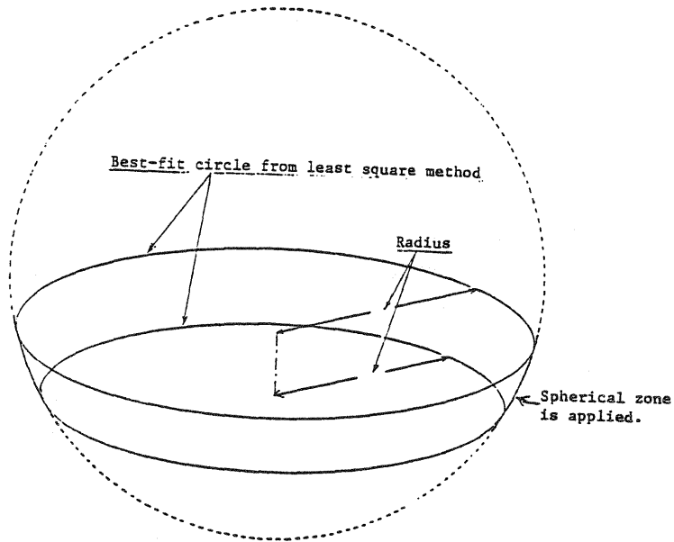
Figure 5: Spherical zone of adjacent two levels
