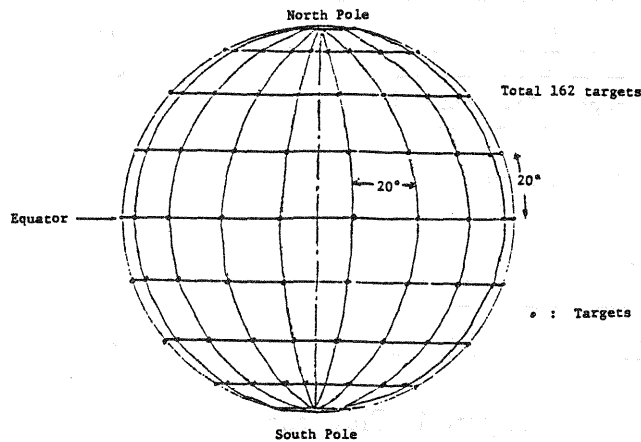
Figure 2: Position and number of targets
