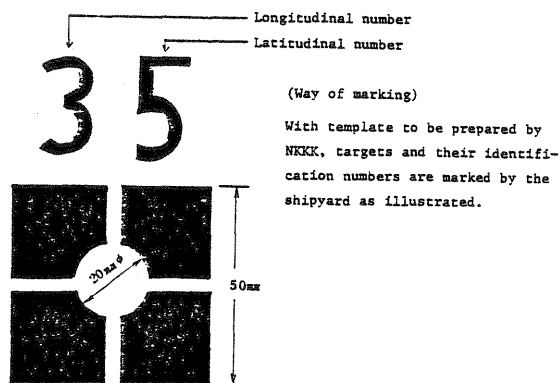
Figure 3: Target and identification number
