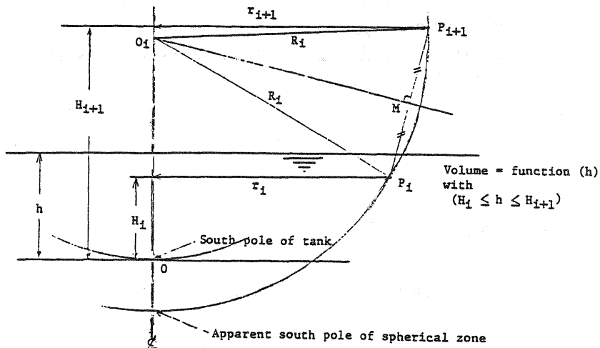
Figure 6: Spherical zone to be applied between level H_i and H_{i+1}
