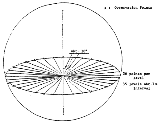
Figure 4: Position & number of observation points
