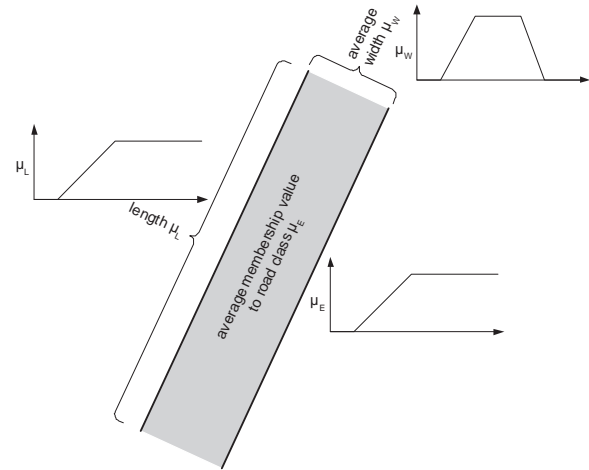
Figure 3: Criteria for the assessment of road hypotheses together with the membership functions for the evaluation of the corresponding fuzzy-values
