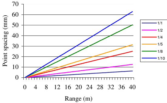
Figure 5. Point spacing at ranges from 0 to 40 meters for different scanning resolutions.
