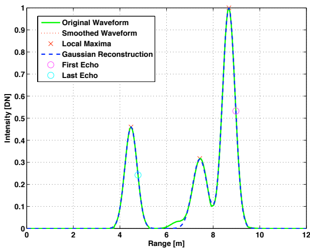
Figure 3: Illustration of Gaussian decomposition for triggering of first and last returns.
