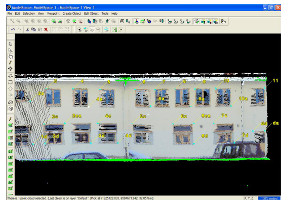
Figure 6. Corrected model, the final result.
