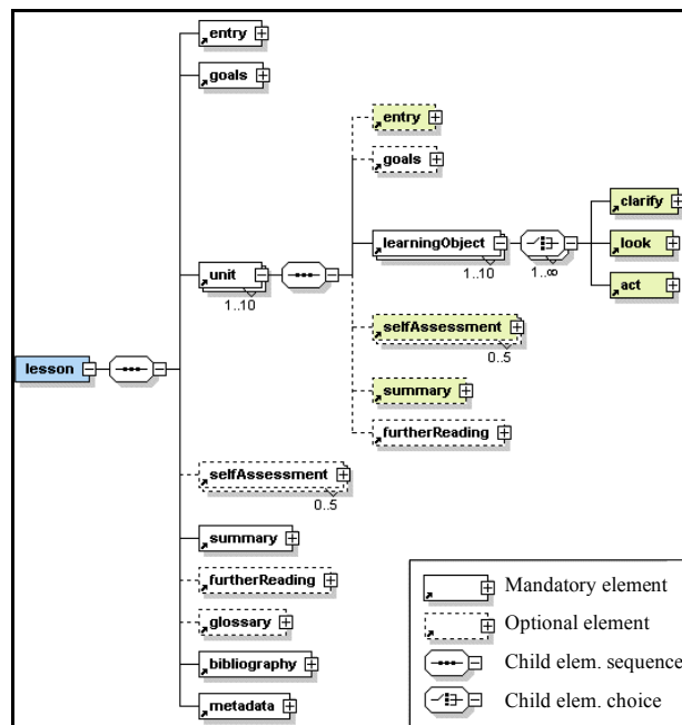
Figure 2: Structure of an eLML lesson
