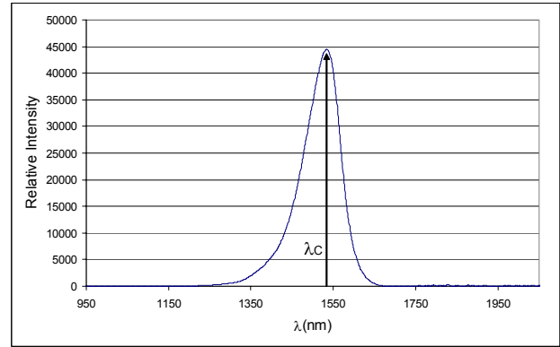
Figure 8. Spectral emission characteristics of the LED centered on 1550 nm. \lambda_c is the central wavelength, \lambda_i and \lambda_f the lower and upper bounds of the peak
