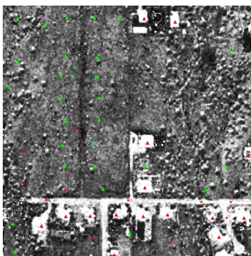
a) hue 2003 (8 bit visualization)
