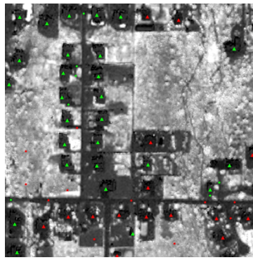
b) NDVI 2005 (8 bit visualization)
