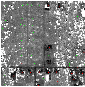
a) NDVI 2003 (8 bit visualization)
