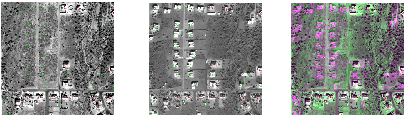
a) PCA 1 2003 (8 bit visualization) triangle: building; circle: surface; green: change; red: no change b) PCA 1 2005 (8 bit visualization) c) change composite (r,g,b:05,03,05)
