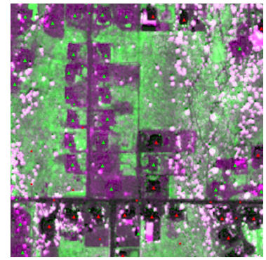
c) change composite (r,g,b:03,05,03)
