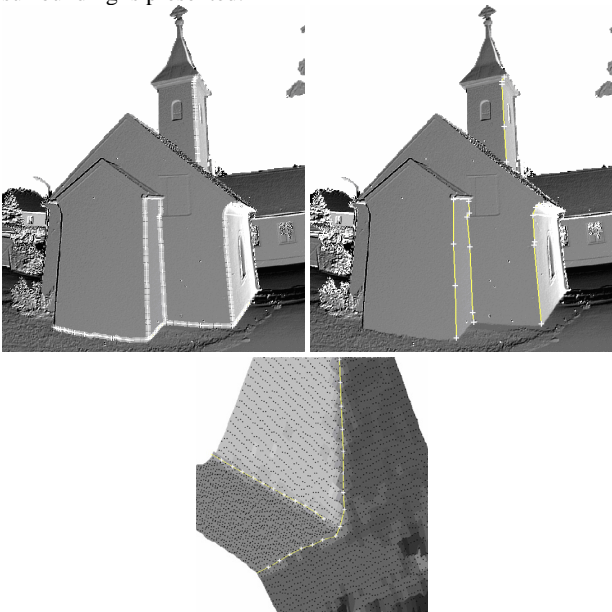
Figure 10: Shading of a 2.5D surface model of the church Gauderndorf in polar domain with structure lines (top left: original structure line, top right: thinned lines according to a max. threshold value). Bottom: 3D detail view of the structure line modelling result with the surrounding point cloud (black).
