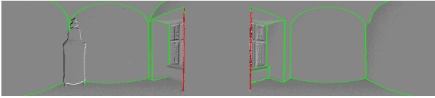
Figure 8: Structure lines (break lines: green, step edges: red) in the polar domain (horizontal: 360°, vertical: 80°) of one scan of the Bergl room acquired with the Riegl scanner LMS-Z420i.
