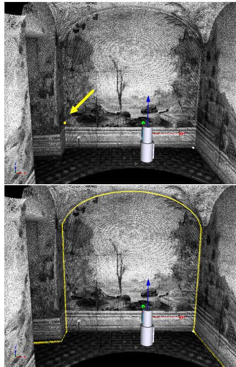
Figure 7: Structure line growing. 3D view of the TLS point cloud recorded in the Bergl room. The point cloud is coloured with the recorded intensity information. The growing process is initialised with the help of one 2D start point (yellow dot, top). The resulting refined structure line (yellow) is displayed at the bottom.
