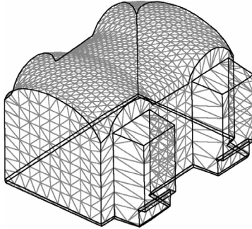
Figure 9: Final geometric room model (Dorninger and Briese, 2005) with structure lines and representative points within the line information.
