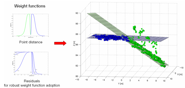
Figure 1: Robust break line modelling of one patch pair using self-adapting weight functions (cf. Briese, 2004b).
