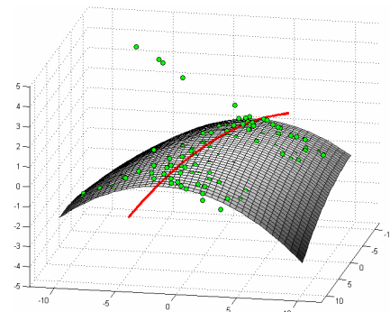
Figure 3: Robust determination of a form line patch based on second order algebraic surfaces.
