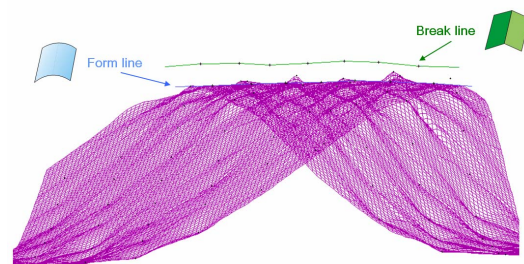
Figure 4: Result of 3D structure line modelling using two different line types. The point cloud is rather describing a form line. Therefore, the estimated break line (green) deviates from the surface interpolated from the TLS points (black dots), whereas the estimated structure line using the form line determination process (blue) represents the linear surface feature in a better way.
