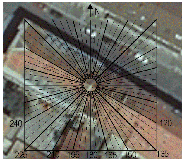
Figure 9. Azimuth determination for object
