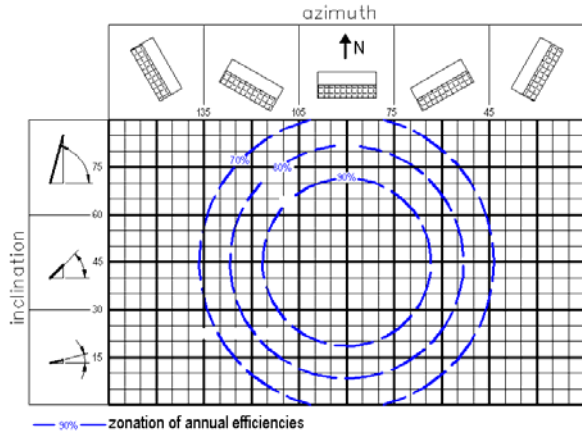
Figure 10. Solar energy as the function of inclination and azimuth
