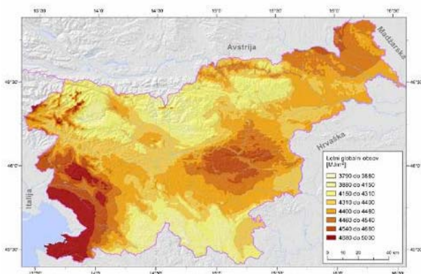
Figure 1. Energy of annual global radiation in Slovenia
