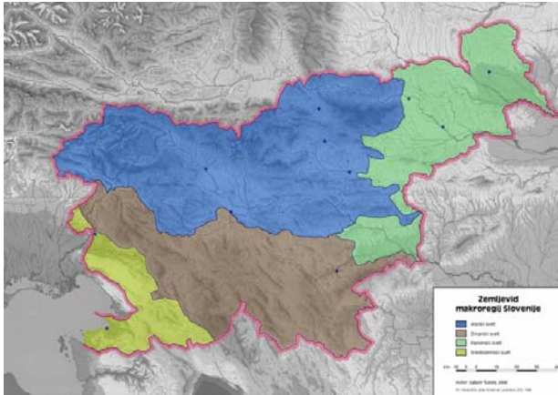
Figure 6. Solar determination radiation regions (alpine, dinaric mountain, panonian basin and Mediterranean region),
