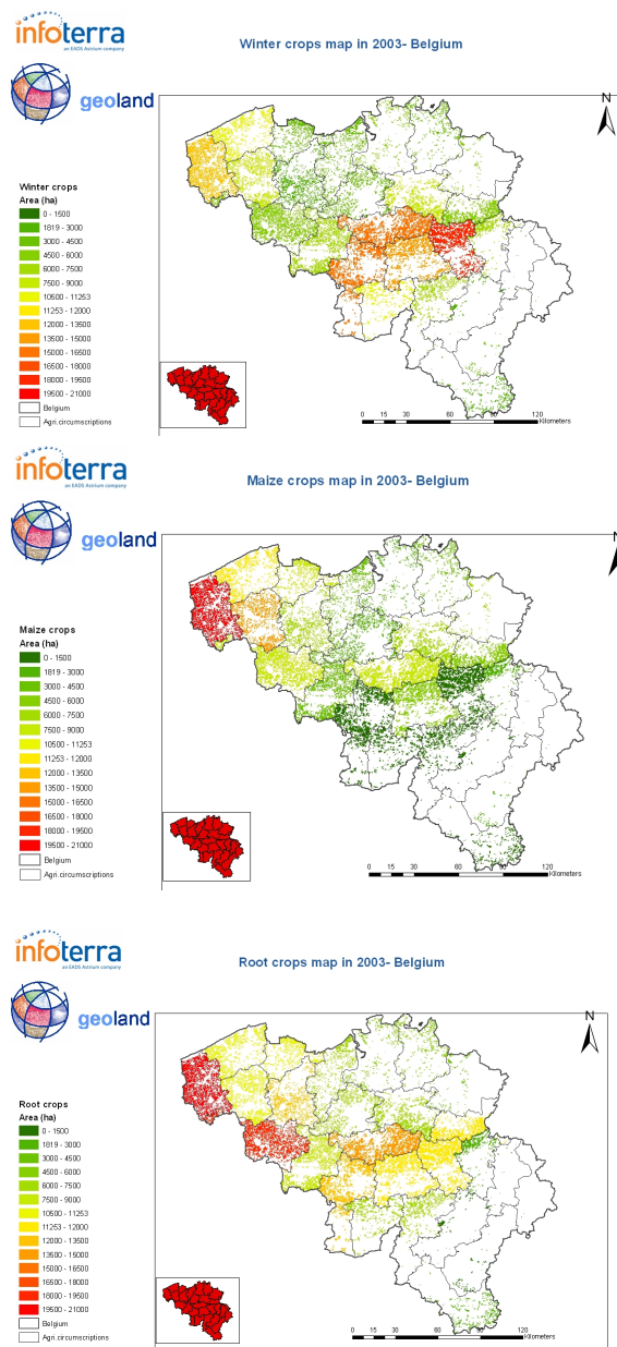
Figure 5-1. Illustration of arable acreages maps on the whole of Belgium in 2003: Winter crops, -Maize crops and Root (sugar beet and potatoes) crops.
