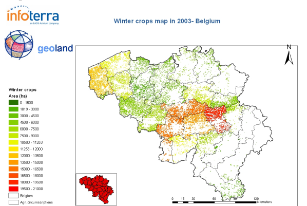
Figure 1. Winter crops acreage maps per agri-circumscription unit in Belgium in 2003.
