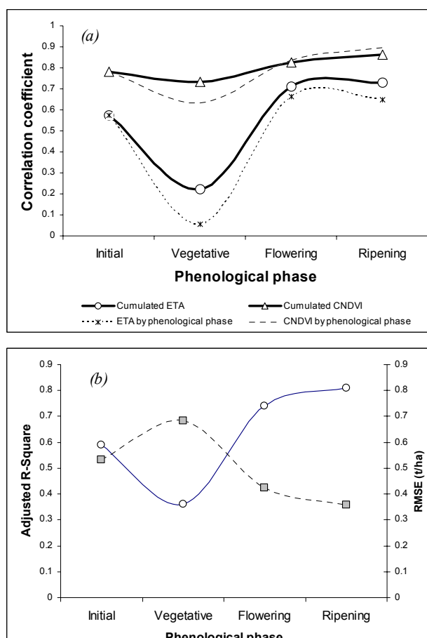
Figure 8 (a) Variation of the correlation coefficient ( r ) with the independent variables cumulated during the whole cycle and cumulated by phenological phases. (b) Variation of adjusted r-square and root mean square error in t/ha of the spectral-agrometeorological model using the cumulated CNDVI and ETA when applying the Jack-knife re-sampling technique.
