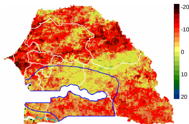
Figure 7: Sorghum difference yield (%), Senegal 2004, GMFS
