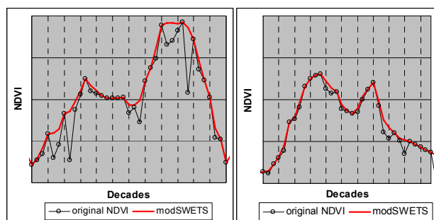
Figure 2. Examples for local profile crop characteristics in Germany with winter cover (left) and in Romania with bimodal NDVI profile (right)
