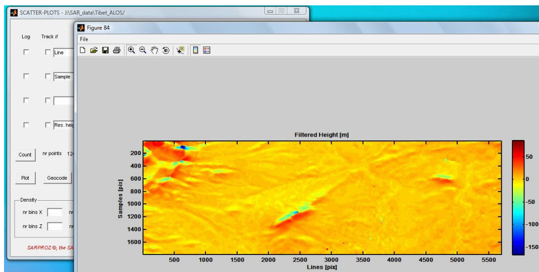
Figure 5. Residual height (w.r.t SRTM) estimated by SARPROZ in the Tibet region from 11 ALOS images. On the background, one of the data visualization modules of SARPROZ. From the image, the railway path can be seen from the left to the right, in the lower part of the plot.
