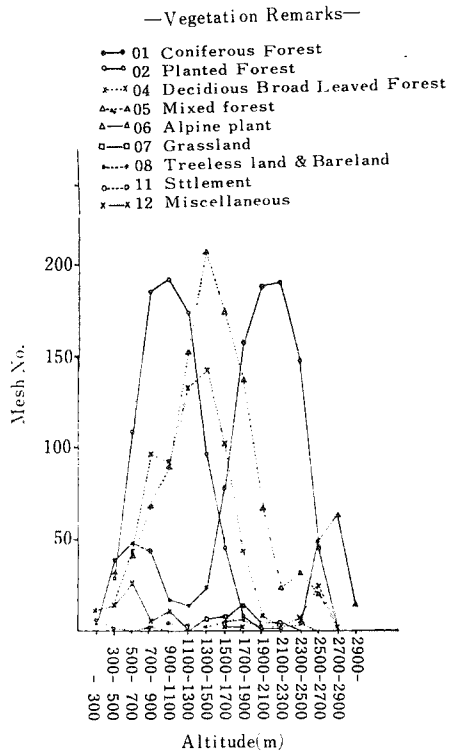
Fig. 25 Altitude vegetation
