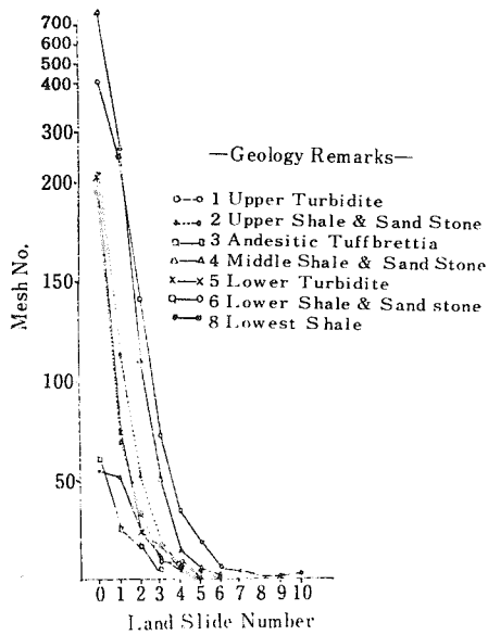
Fig. 27 Land slide-geology
