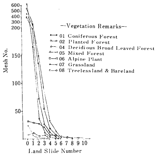
Fig. 28 Land slide-vegetation
