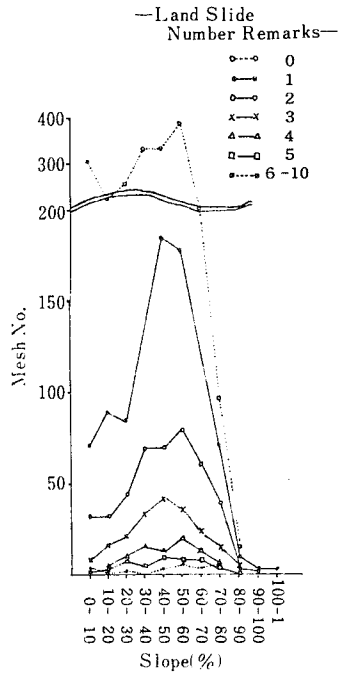
Fig. 26 Land slide-slope
