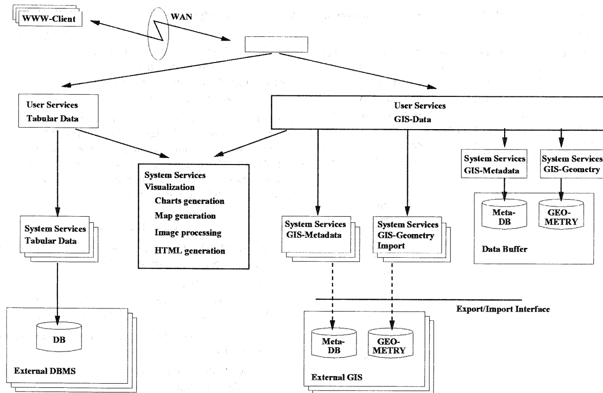
Figure 2: GIS/Graphics architecture
