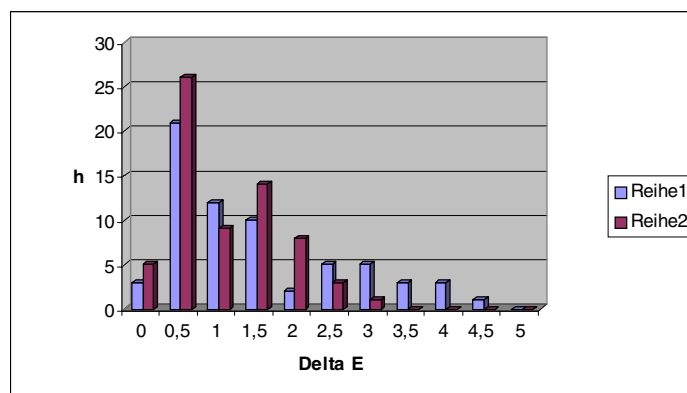
Figure 2. Spread of \Delta E
