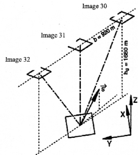
Figure 4: Geometric situation of image acquisition and illumination, real images
