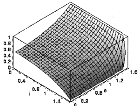
Figure 3: The Lommel-Seeliger reflectance model
