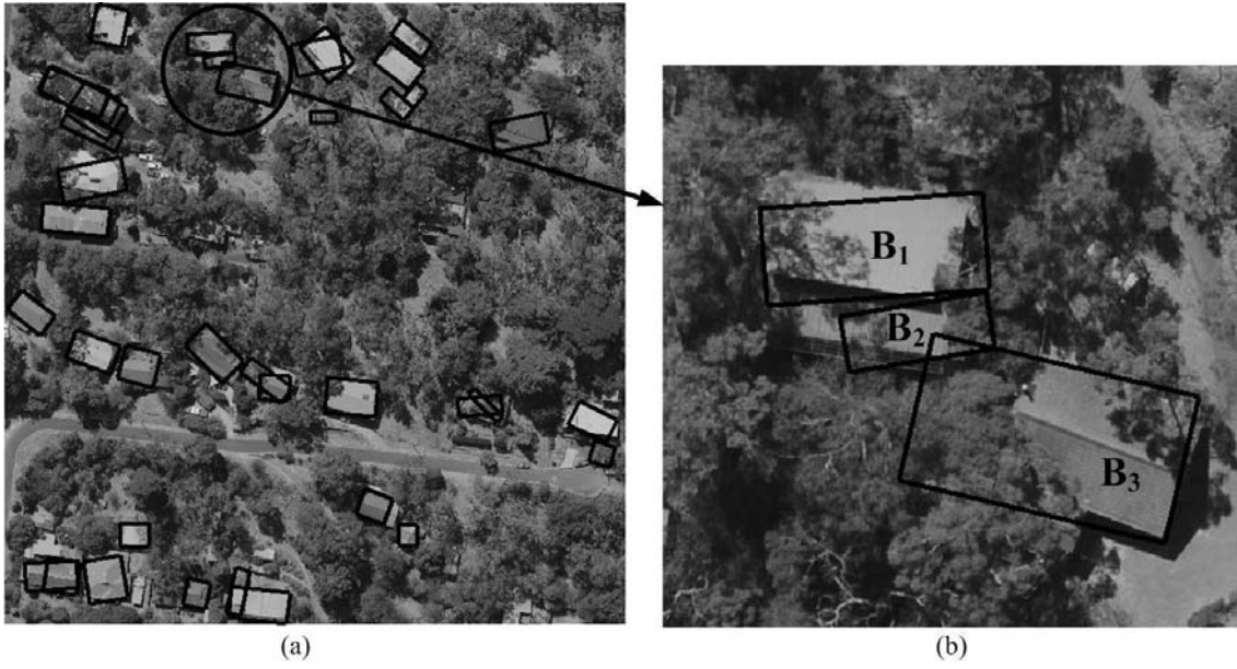
Figure 16. Building detection by the improved detector on a scene from Knox.
