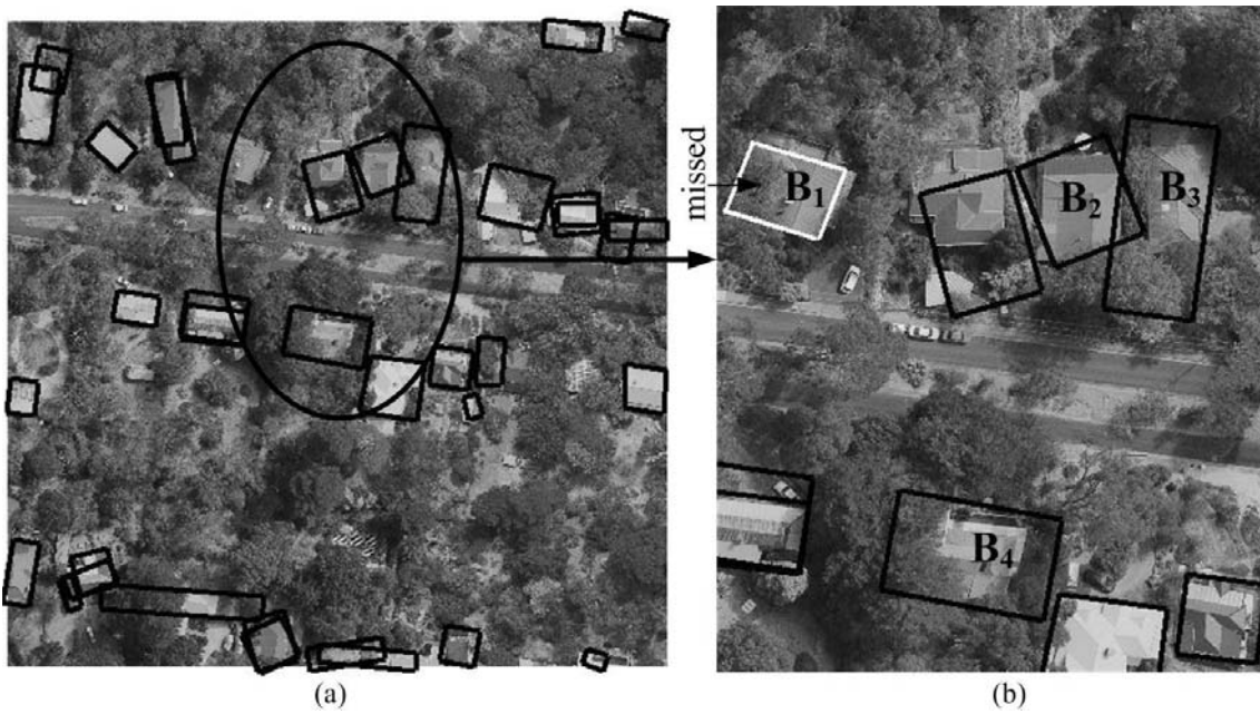
Figure 17. Building detection by the improved detector on a second scene from Knox.
