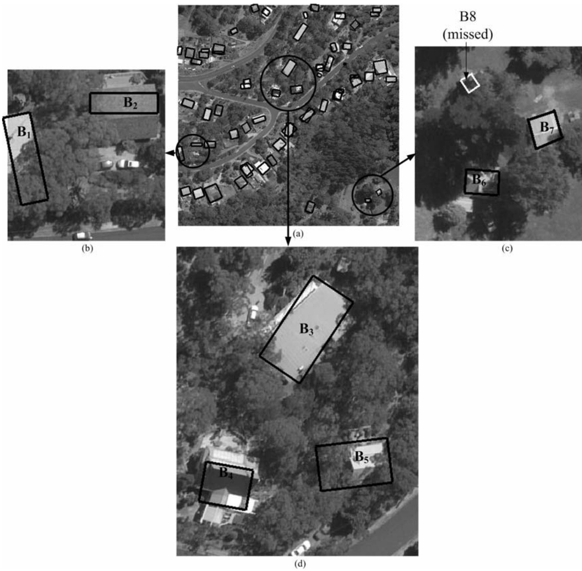
Figure 15. Building detection by the improved detector on a second scene from Hobart.
