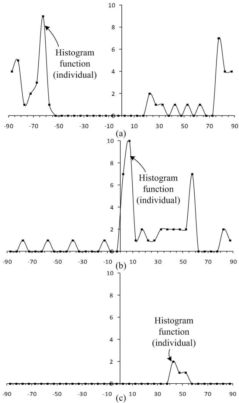
Figure 9. Gradient histogram functions (individual) for candidates (a) B_1 , (b) B_2 and (c) B_3 in Figure 7b: x -axis is in degrees and y -axis is in pixels (bin heights). Two bins at \pm 90^\circ basically form one bin, because lines in these two bins are perpendicular to the x -axis and reside above and below the x -axis. Therefore, when we have peaks at either of these bins, we accumulate their heights to form a single peak.
