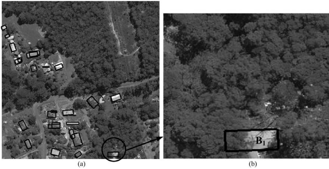
Figure 14. Building detection by the improved detector on a scene from Hobart.
