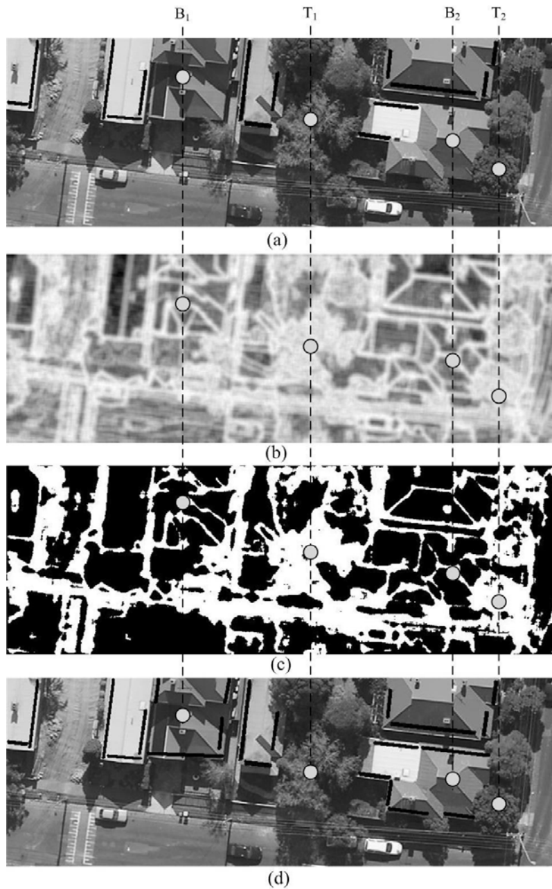
Figure 4. Detection of green buildings: (a) the NDVI information alone missed green buildings B_1 and B_2 , (b) entropy image for the scene in (a), (c) entropy mask from (b), and (d) combined NDVI and entropy information is able to detect the two green buildings. In (a) and (d), black lines represent detected buildings. In (b) and (c), while black pixels represent low entropy areas, white pixels represent high entropy areas.
