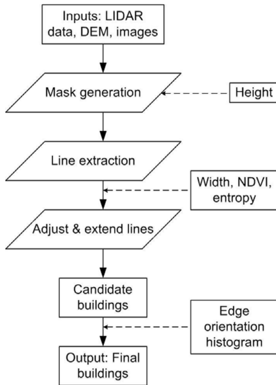
Figure 2. Flow diagram of the improved building detection technique.
