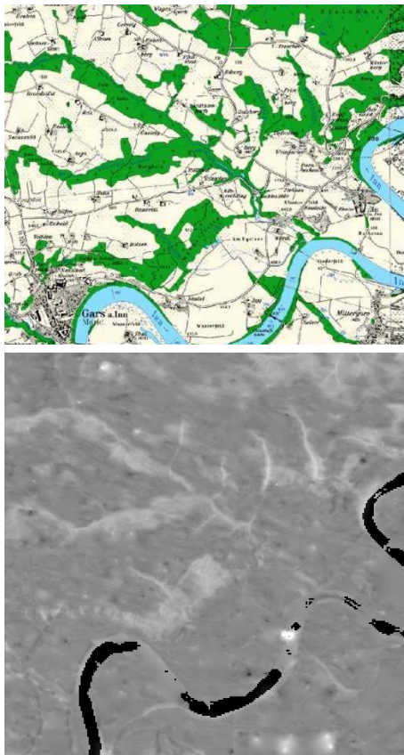
Figure 4. Lower part: Difference DEM (SPOT DEM – Reference DEM): Bright: forest areas and some blunders, the black parts have no value in the reference DEM. Upper part: Map of the same
