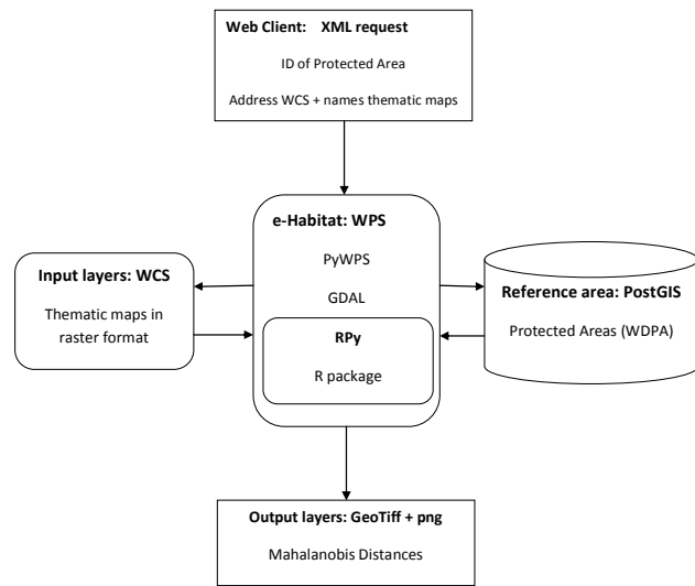
Figure 2. Flowchart of eHabitat 1.0. The WPS receives an XML request with the ID of a protected area available from the World Database of Protected Areas (IUCN-WCMC) and 3 thematic maps in a raster format. The HRI is computed for the protected area within a defined bounding box and the final results released in a GeoTIFF and png format.
