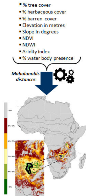
Figure 1. p -value grid (insert, lower left) showing probabilities, in the Zambesian ecoregion, to find similar habitats to the one found in the Kafue national park (Zambia). The HRI is computed here using the 9 thematic layers indicated on top. NDVI = Normalized Difference Vegetation Index, NDWI = Normalized Difference Water Index (NDWI).
