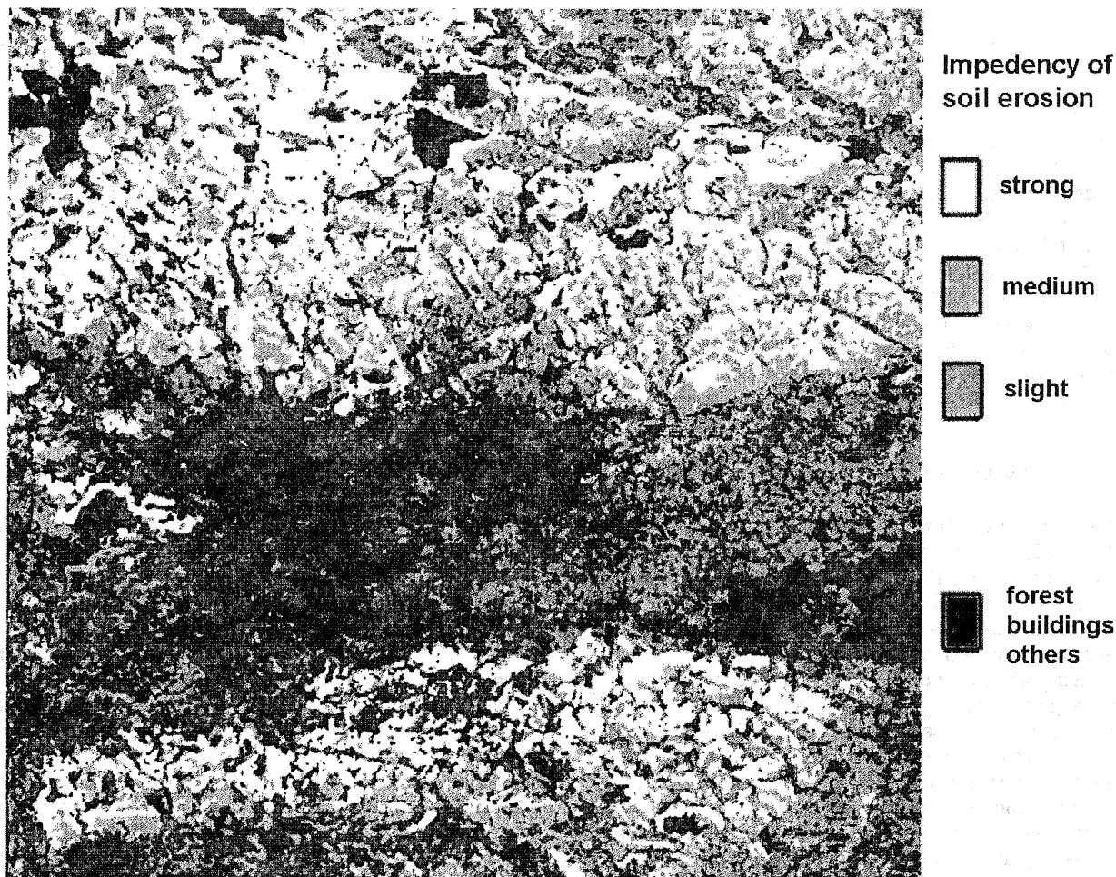
Fig.4. Soil erosion potential map
