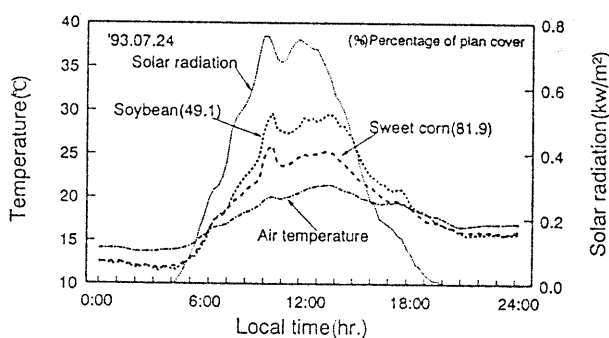
Fig. 7(c) Daily changes of canopy temperature, air temperature and solar radiation for crop fields (on July 24, 1993).
