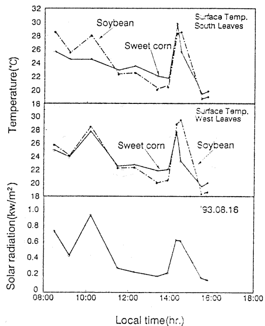
Fig. 4 Surface temperature at the upper-most leaf.
