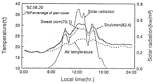
Fig. 7 (a) Daily changes of canopy temperature, air temperature and solar radiation for crop fields (on August 30, 1992).
