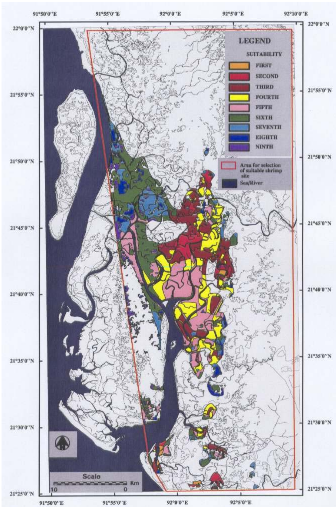
Figure 3. Map showing sites in order of suitability of shrimp farming in Cox's Bazar study area.
