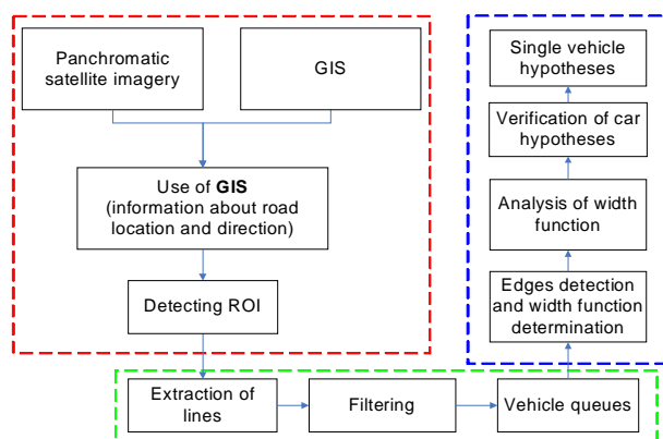
Figure 2. Overall structure
