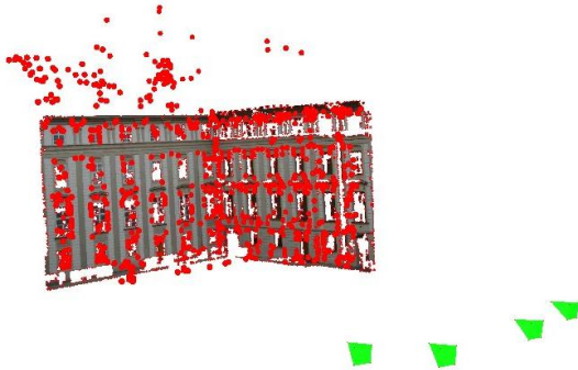
Figure 4: The two dominant planes restricted to the areas classified to be on the plane together with the 3D points (red) and the cameras (green pyramids)
