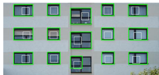
Figure 9: Result of MCMC – hypotheses (white box) and windows (green box)
