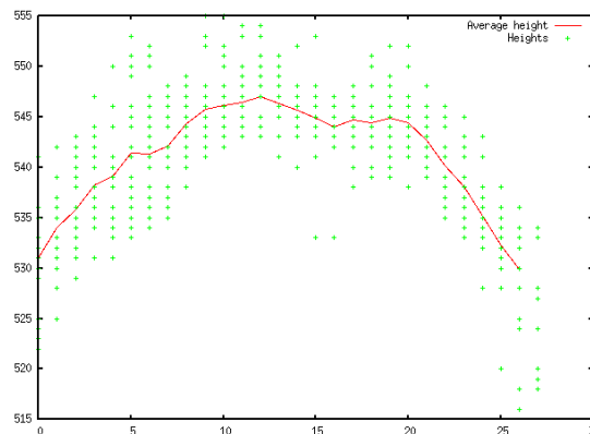
Figure 14. Statistics of DSM heights from object 2 across roof direction (green dots: DSM values all along the roof, red line: averaged profile)
