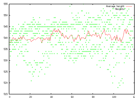
Figure 15. Statistics of DSM-heights from object 2 along roof direction (green dots: DSM values all across the roof, red line: averaged profile)
