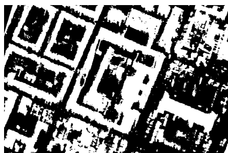
Figure 4. High objects mask calculated from the DSM and the derived DTM applying a height threshold of 4 m (section 600 m × 400 m)
