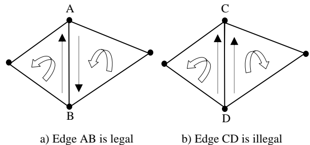
Figure 2. Detection of illegal edges
