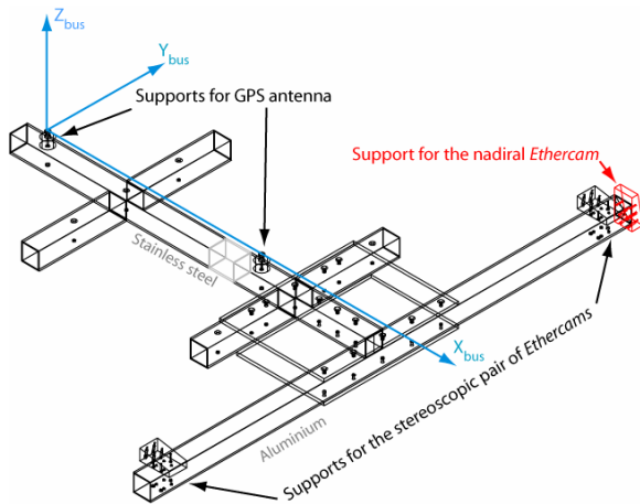
Figure 5. Sensor-supporting structure
