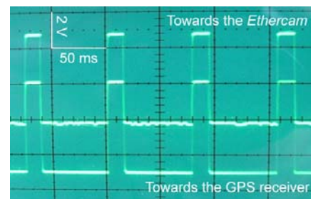
Figure 3. Simultaneity of TTL-compatible signals reaching a GPS receiver and the EthernCam
