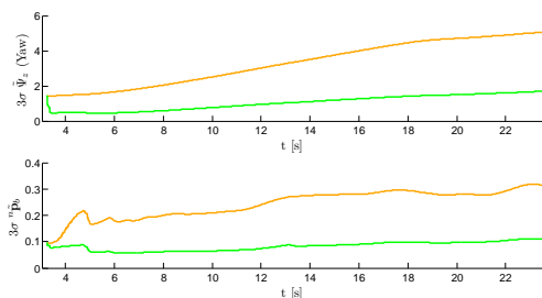
(c) Yaw angle and position covariance bounds
