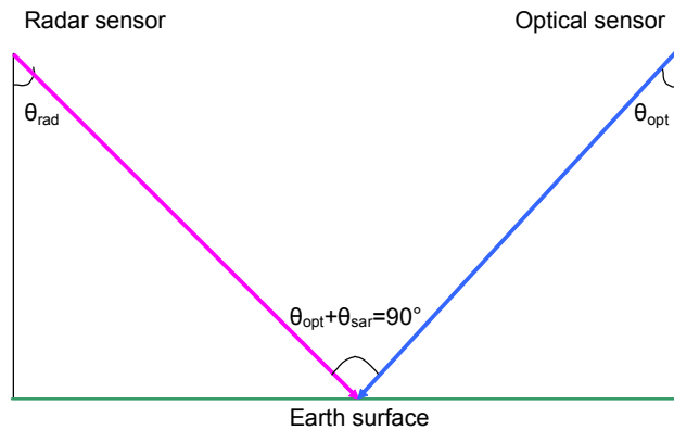
Figure 3. Proposed optimal and radar sensor formation is illustrated. A sum of look angles should give 90^\circ .
