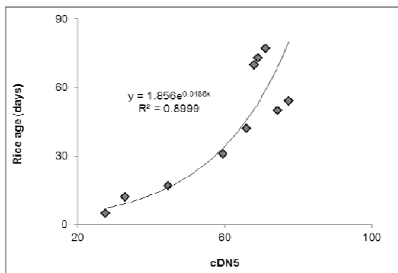
Figure 2. Relationship between rice cDN of Landsat ETM+ and rice age of Band 5.
