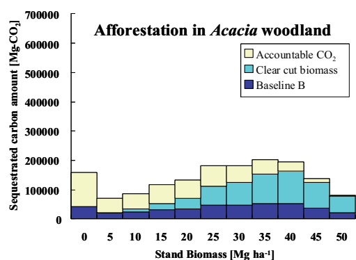
Figure 4. Sequestered carbon amount by CO 2 conversion when afforestation sites were established in bare ground, the vegetation transition area and Acacia woodland when baseline scenario B was adopted for calculating Equation (1).
