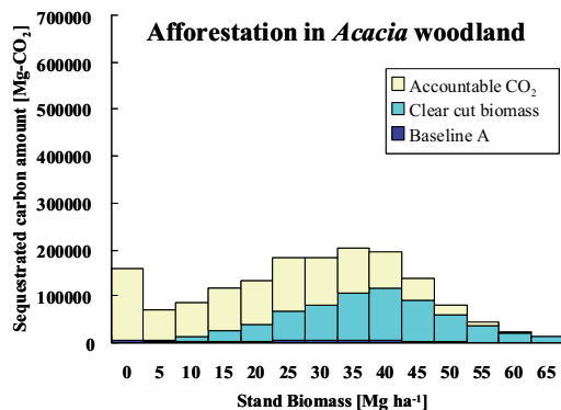
Figure 3. Sequestered carbon amount by CO 2 conversion when afforestation sites were established in bare ground, the vegetation transition area and Acacia woodland when baseline scenario A was adopted for calculating Equation (1).
