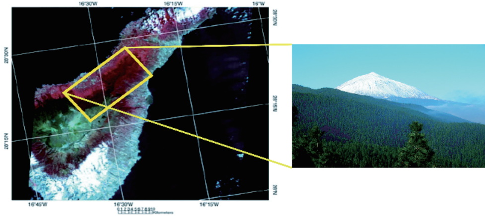
Figure 1. ASTER colour composite of Tenerife Island for April 16, 2008. RGB components are ASTER bands 3 (0.81 μm), 2 (0.66 μm) and 1 (0.56 μm). Zoom image corresponds to a panoramic view of the coniferous forest in the northern side of Tenerife.
