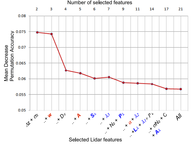
Figure 3: Iterative elimination Lidar feature selection.
