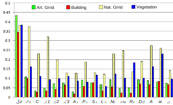
Figure 5: Variable importance per class - 3 \times 3 window size
