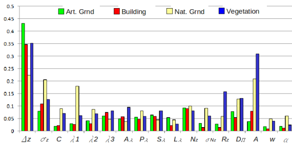
Figure 6: Variable importance per class - 5 \times 5 window size
