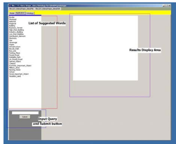
Figure 3: User Interface Application
