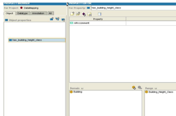
Figure 6: Building_Height_Class is related with Building by owl:objectProperty (in Protégé)
