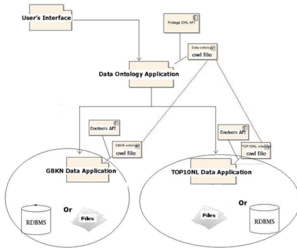
Figure 2: Prototype system architecture
