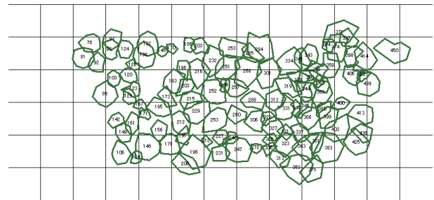
Figure 11: The projected on-ground map of measured 102 canopy trees.
