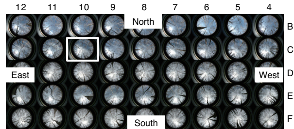
Figure 4: The canopy photos on 22 April 2006.
