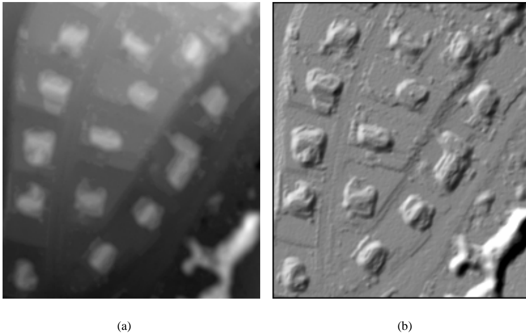
Figure 3: DSM of the residential ROI: (a) intensity “image” of the model; (b) embossed version of this image.
